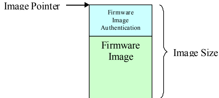
Figure 62. Firmware Image with Authentication Support
