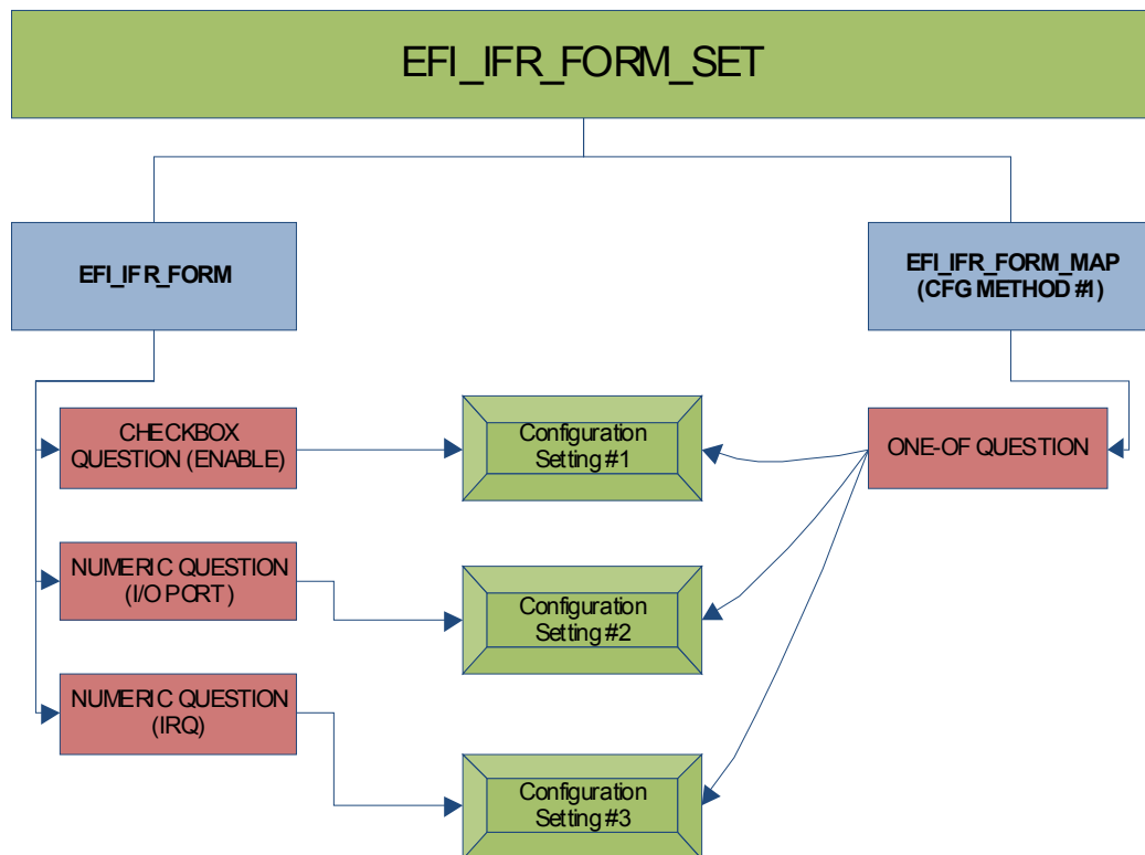
Figure 109. EFI IFR Form Set question changes
