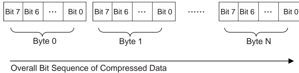
Figure 55. Bit Sequence of Compressed Data
