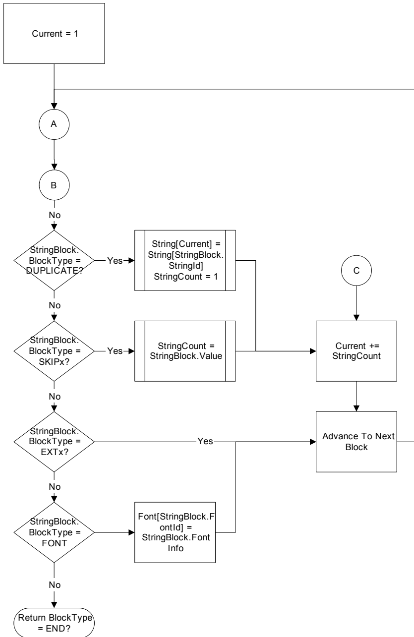
Figure 113. String Block Processing: Base Processing
