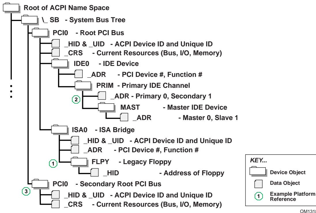
Figure 126. Partial ACPI Name Space for Example System
