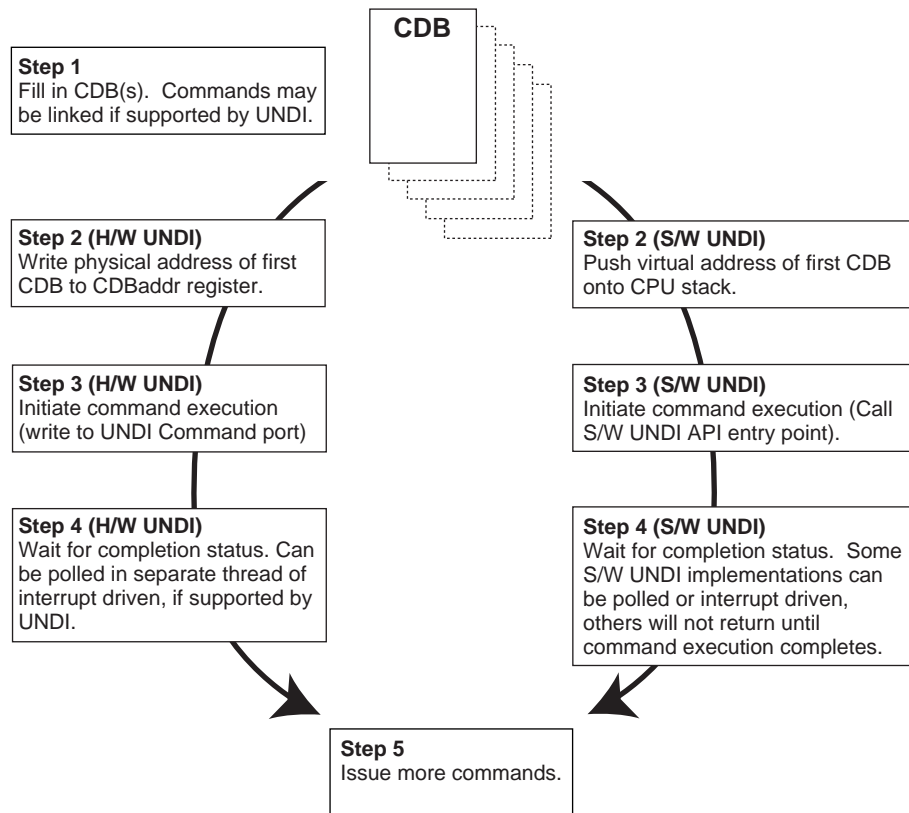
Figure 130. Issuing UNDI Commands
