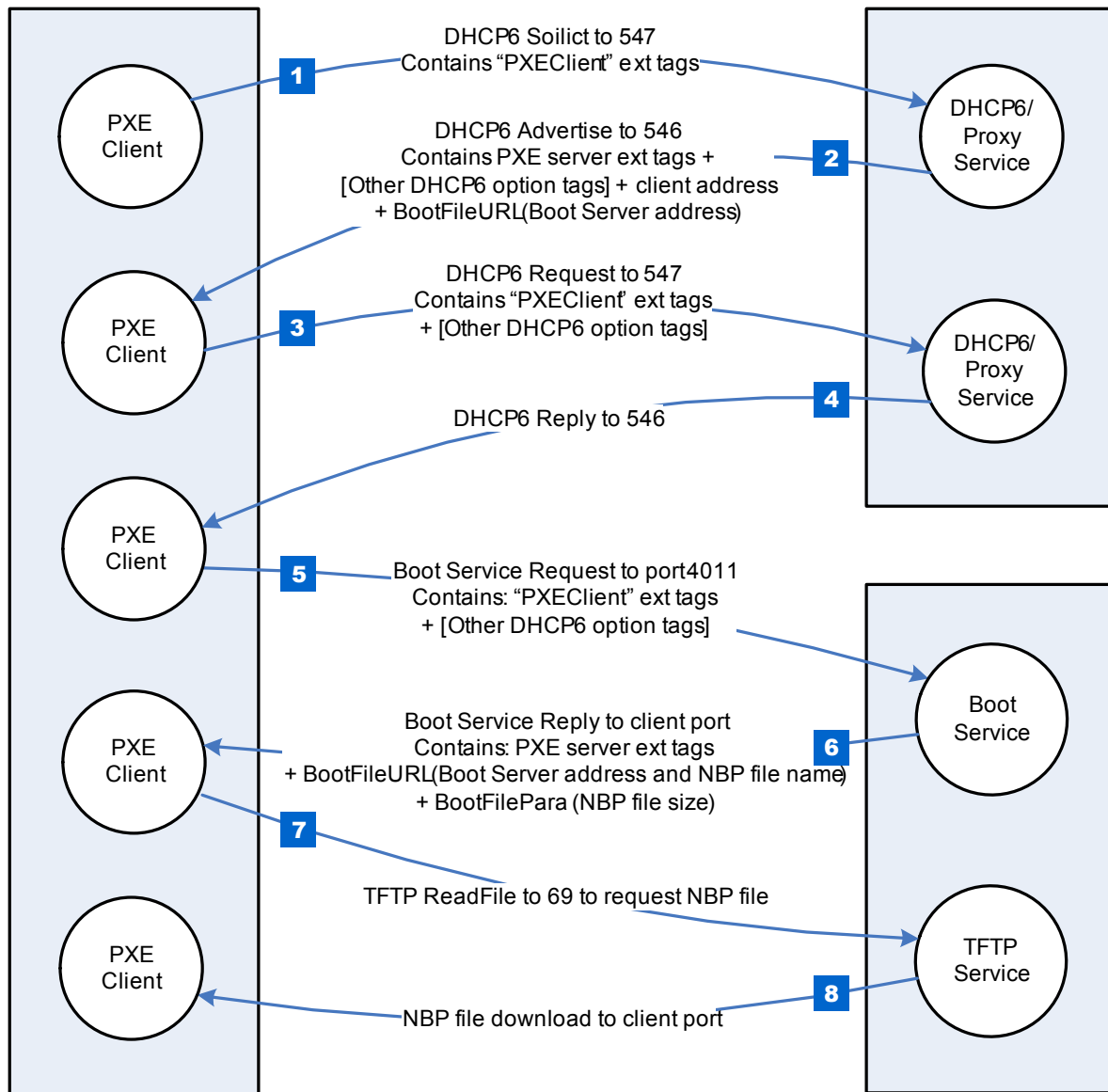
Figure 66. IPv6-based PXE boot
