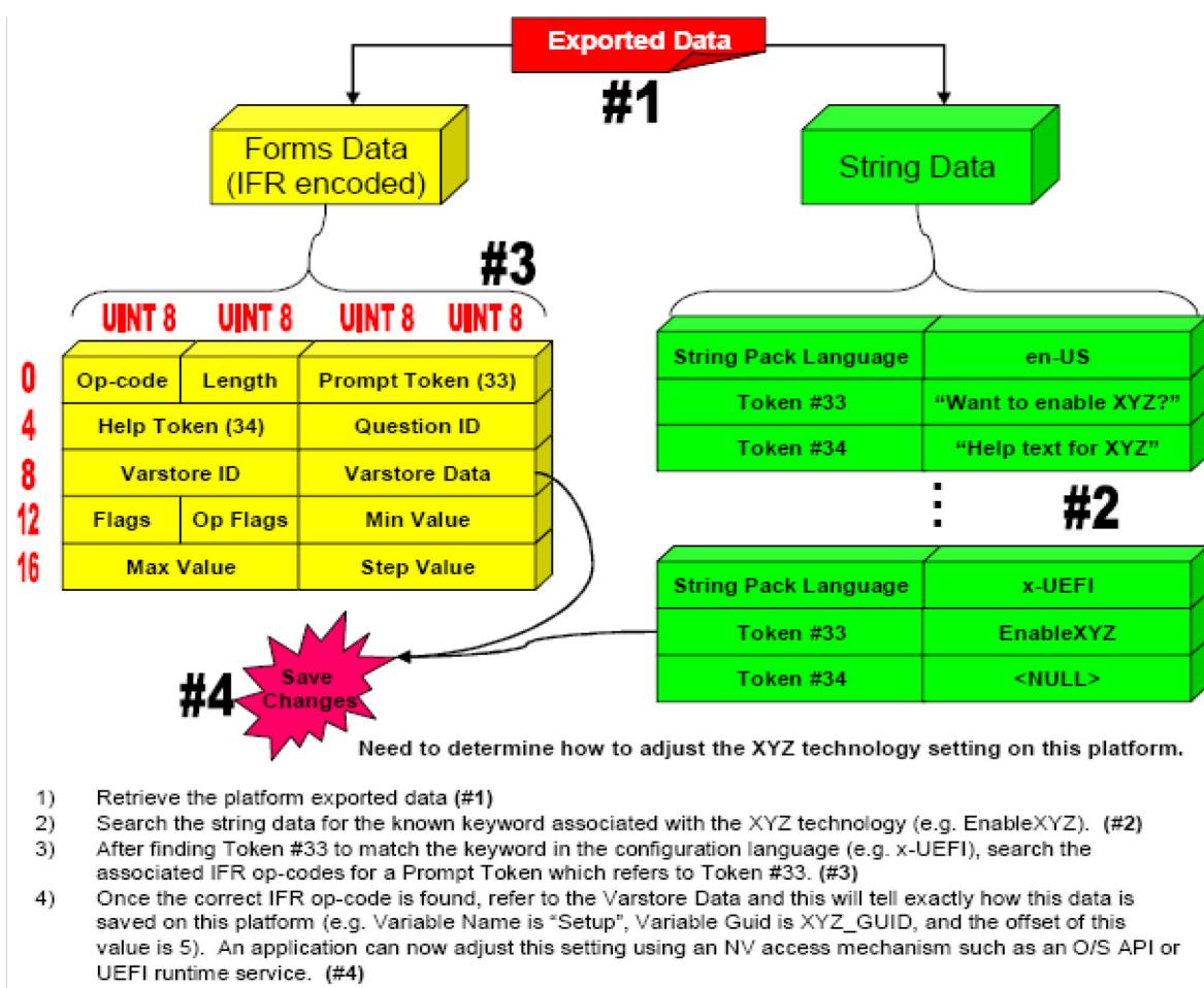
Figure 102. Standard Application Obtaining Setting Example
