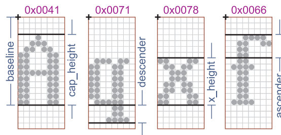
Figure 93. Font Description Terms
