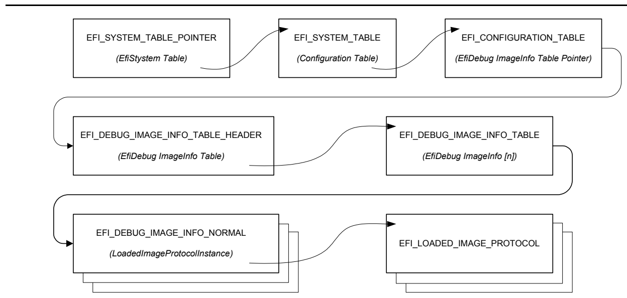
Figure 54. Debug Support Table Indirection and Pointer Usage
