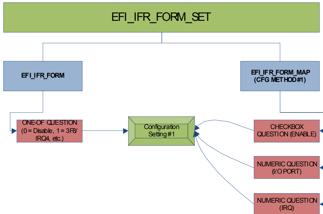
Figure 108. EFI IFR Form set configuration
