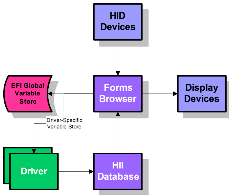
Figure 75. Platform Configuration Overview
