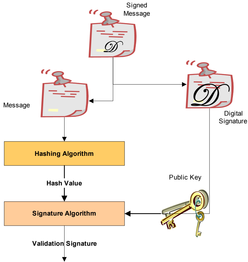
Figure 70. Verifying a Digital Signature
