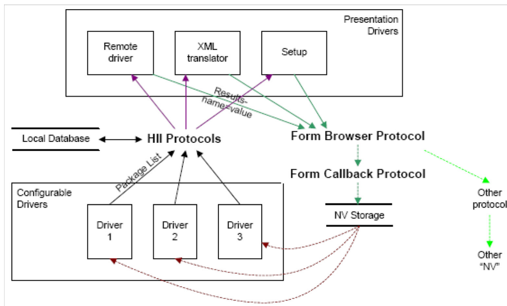
Figure 107. Managing Human Interface Components
