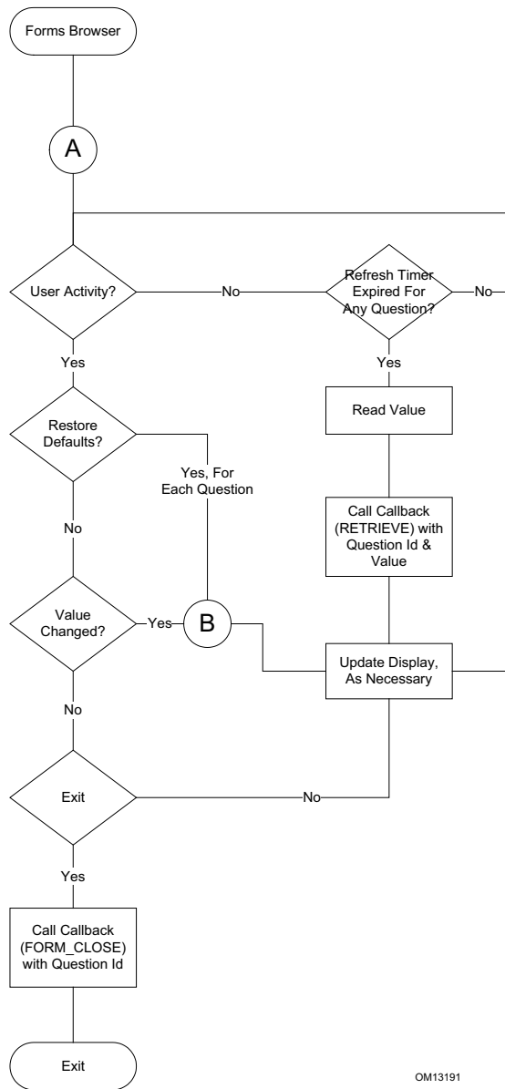
Figure 104. Typical Forms Processor Decisions Necessitating a Callback (2)
