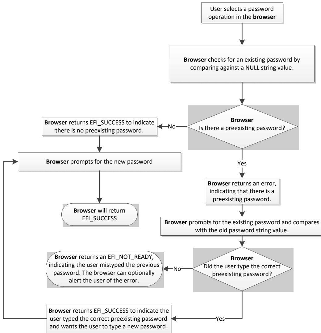
Figure 122. Password Flowchart (part two)
