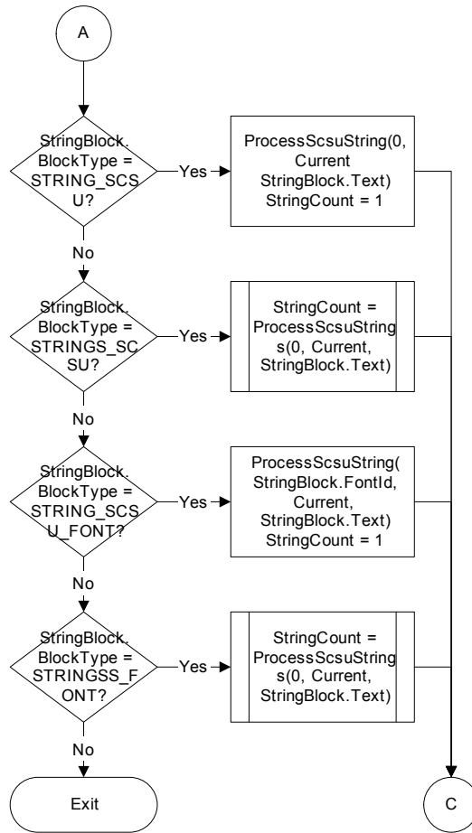
Figure 114. String Block Processing: SCSU Processing
