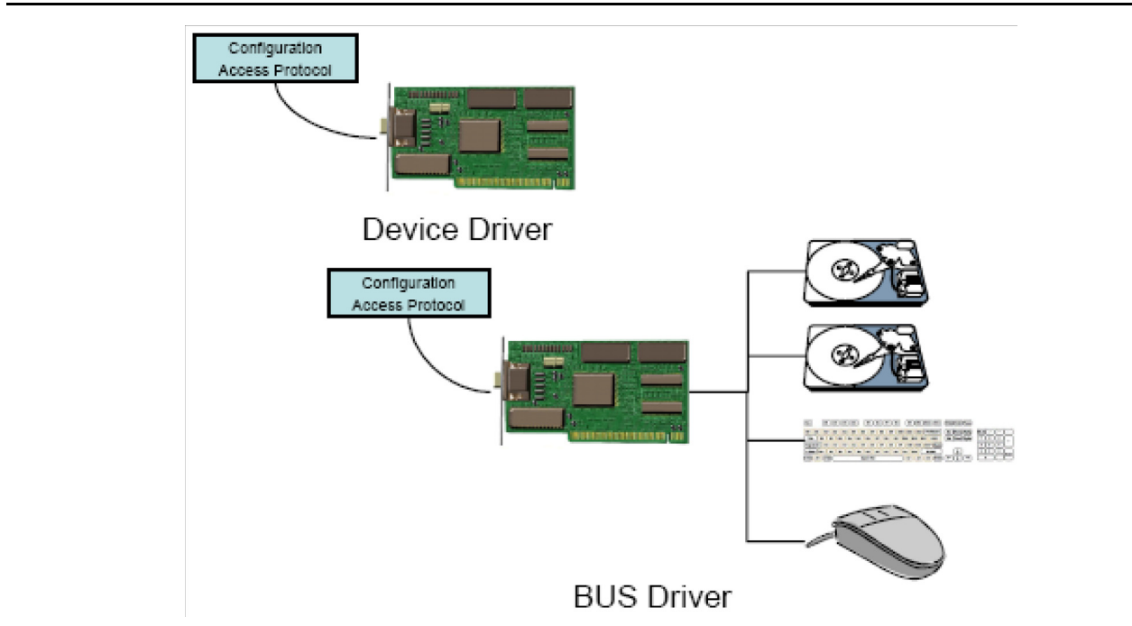
Figure 106. Driver Model Interactions
