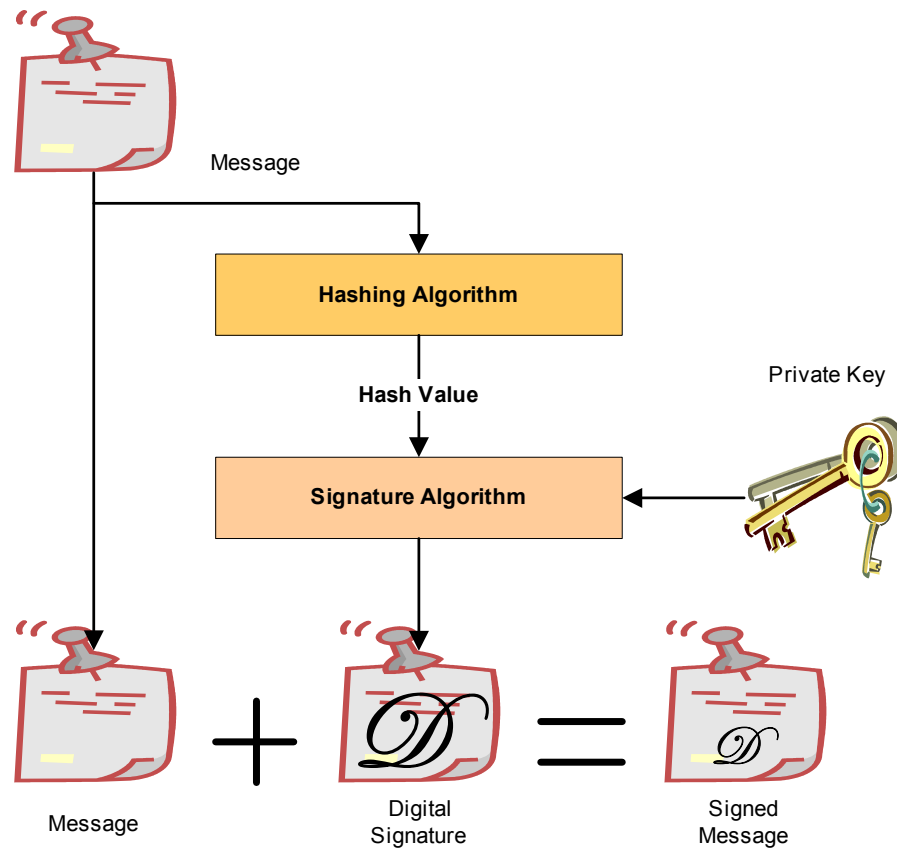
Figure 69. Creating A Digital Signature
