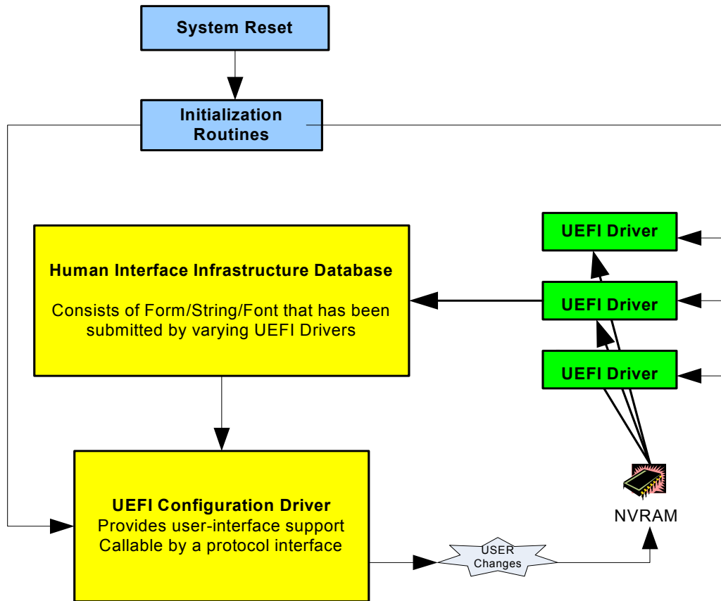
Figure 100. Storing Configuration Settings
