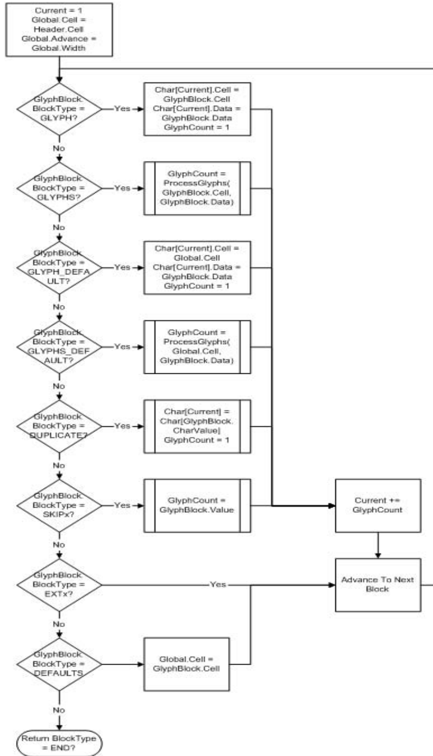
Figure 111. Glyph Block Processing
