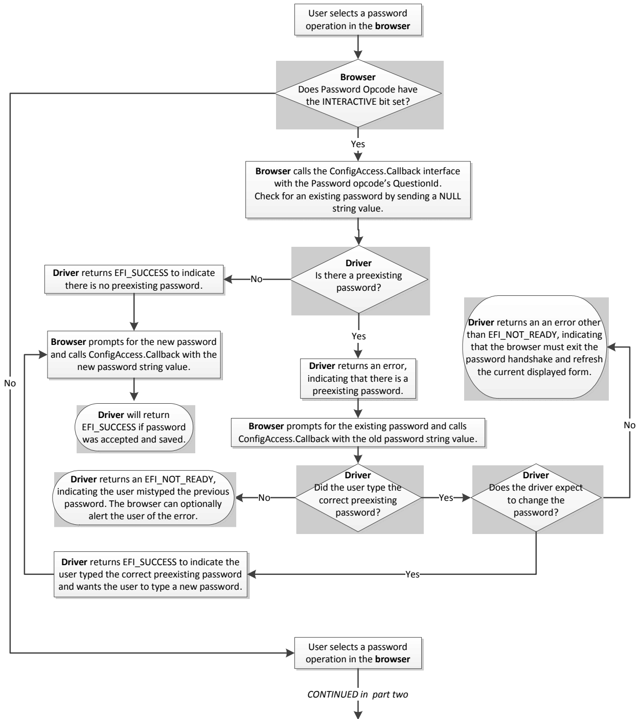
Figure 121. Password Flowchart (part one)
