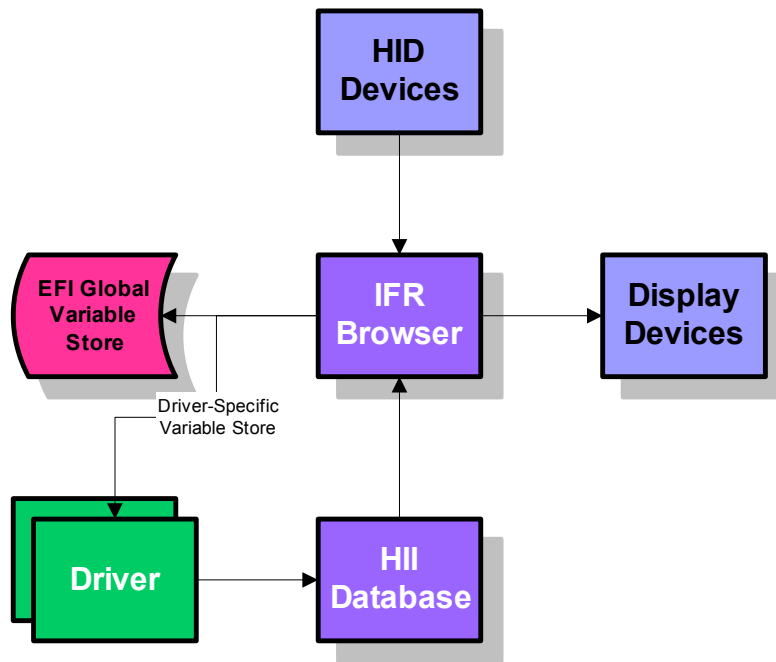
Figure 88. Platform Configuration Overview
