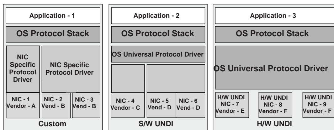
Figure 128. Network Stacks with Three Classes of Drivers
