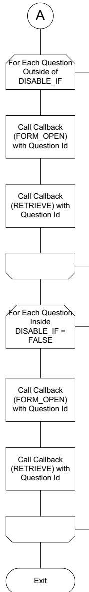
Figure 103. Typical Forms Processor Decisions Necessitating a Callback (1)
