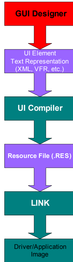
Figure 78. Creating UI Resources With Intermediate Source Representation
