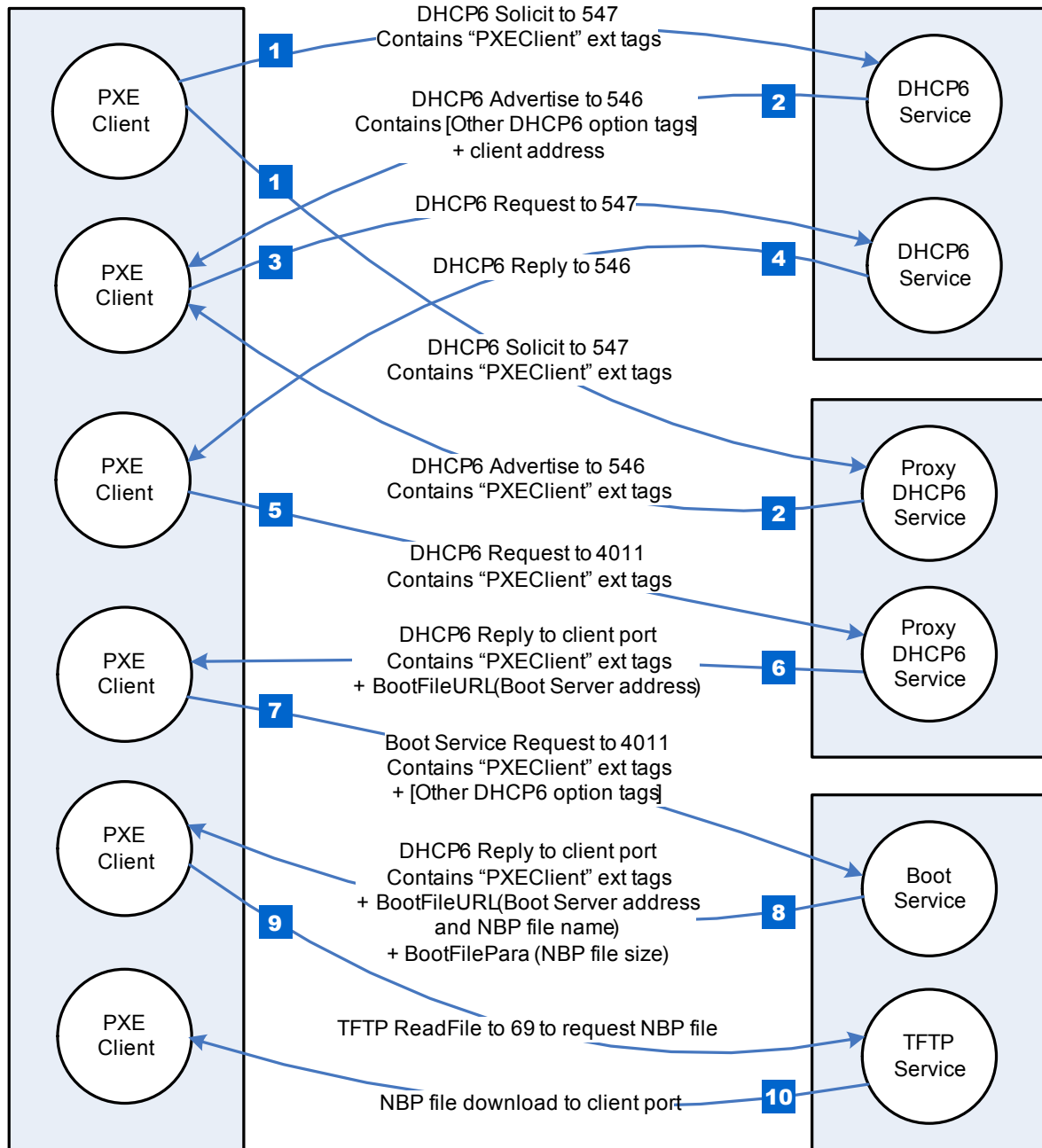
Figure 68. IPv6-based PXE boot (DHCP6 and ProxyDHCP6 reside on the different server)
