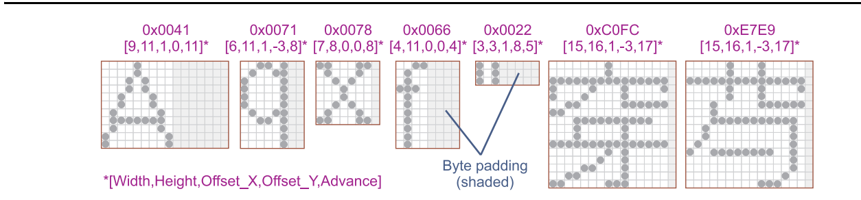
Figure 96. Proportional Font Parameters and Byte Padding
