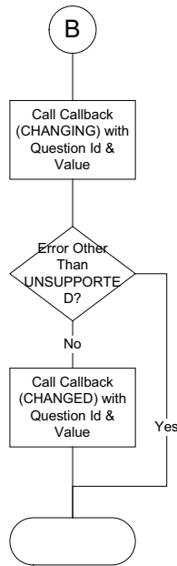
Figure 105. Typical Forms Processor Decisions Necessitating a Callback (3)
