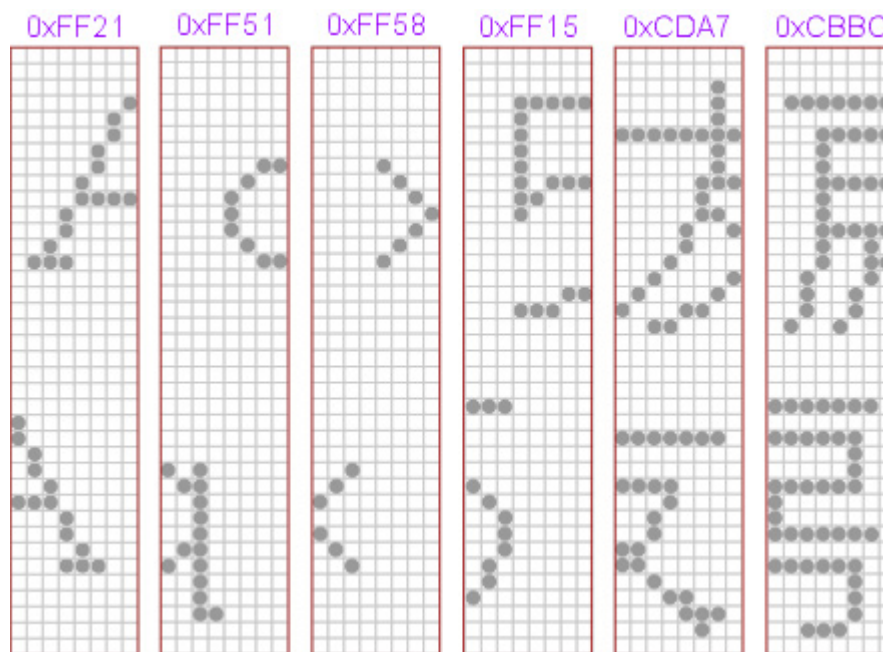
Figure 95. Font Structure Layout
