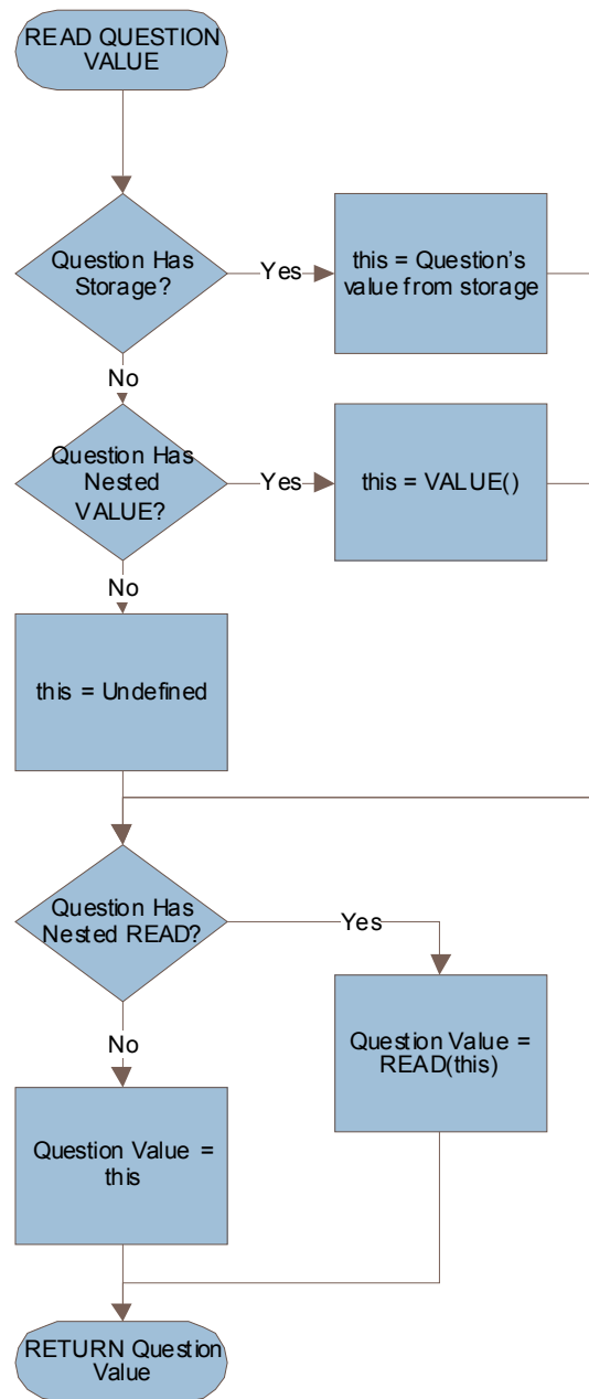
Figure 89. Question Value Retrieval Process
