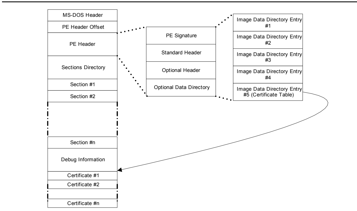
Figure 71. Embedded Digital Certificates
