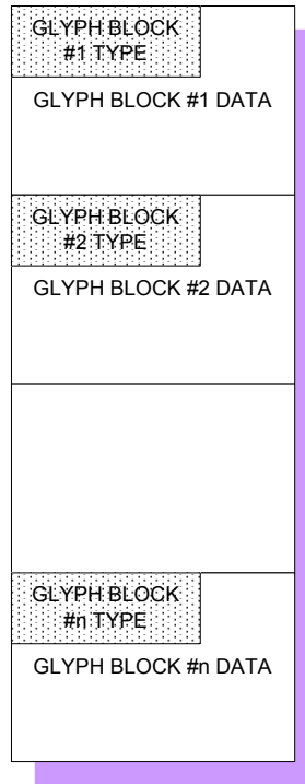
Figure 110. Glyph Information Encoded in Blocks
