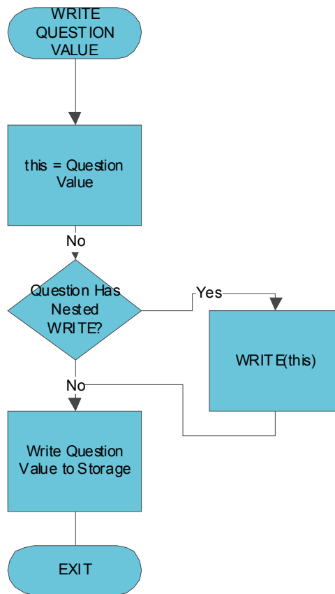
Figure 90. Question Value Change Process
