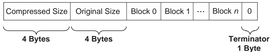
Figure 56. Compressed Data Structure
