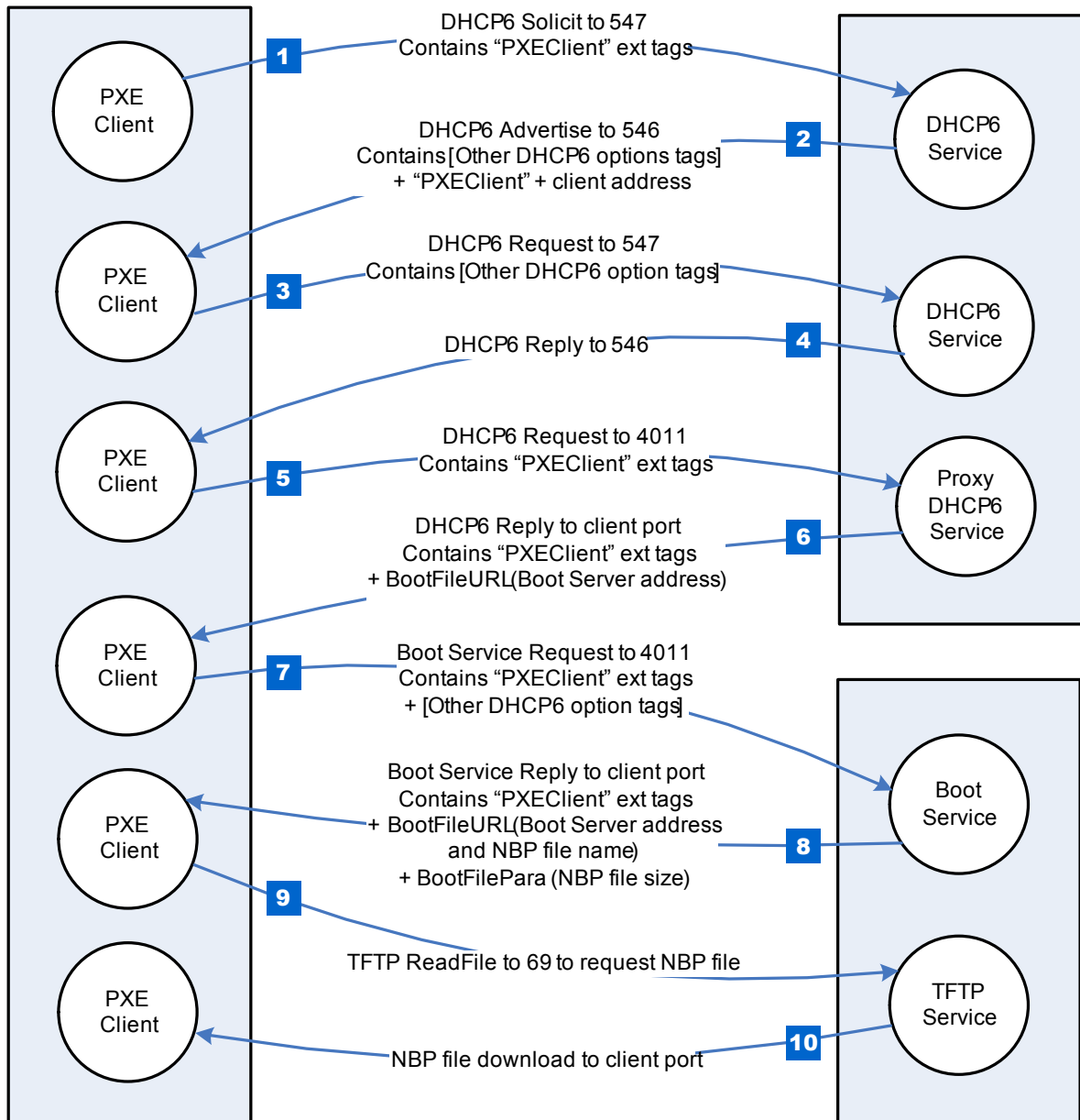
Figure 67. netboot6 (DHCP6 and ProxyDHCP6 reside on the same server)
