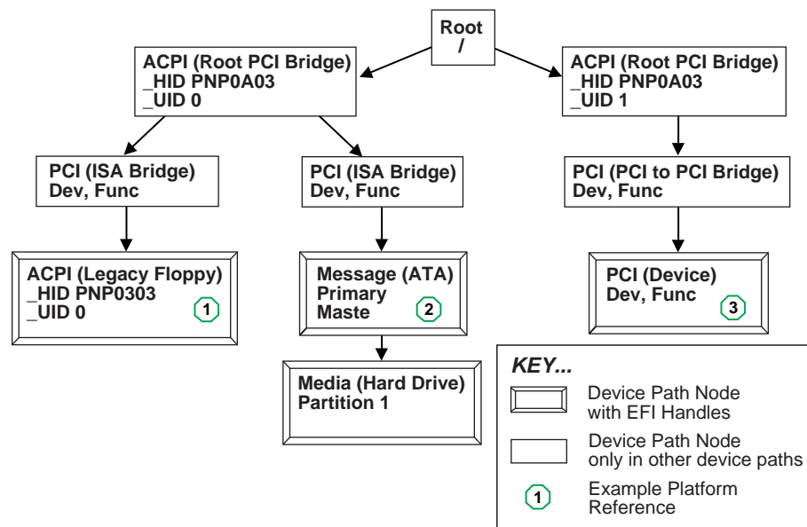
Figure 127. EFI Device Path Displayed As a Name Space
