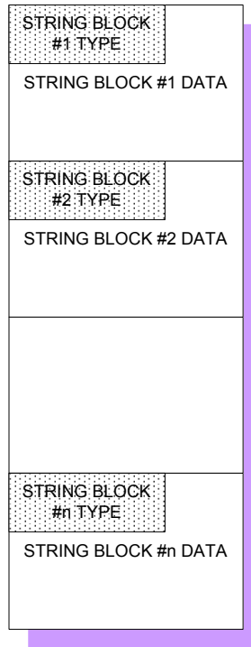
Figure 112. String Information Encoded in Blocks
